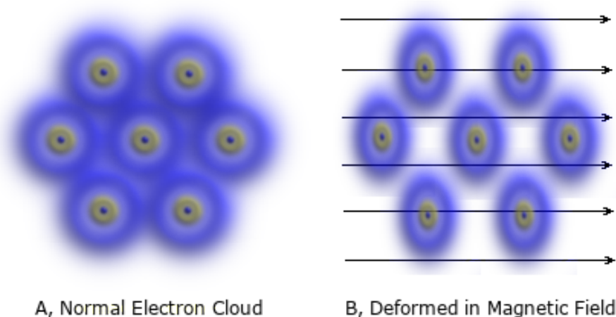
Figure 7. Superconductivity is destroyed in a magnetic field above a critical intensity. (A) In a weak or absence of an external magnetic field, the applied field can be completely canceled by the internal field in a superconductor due to the Meissner effect. The electron clouds of valence electrons extend normally into electron tunnels. Superconductivity may withstand a magnetic field up to a critical intensity. (B) However, an external field over the critical intensity cannot be completely offset due to the limit of the critical current density. Orbital electrons are deflected by the Lorentz force in the remaining field and divert their orbiting plane in the direction perpendicular to the external field. This action compresses the electron clouds like squashed lanterns. The deformation of orbitals causes the valence electrons to withdraw from the electron tunnels, destroying superconductivity.
