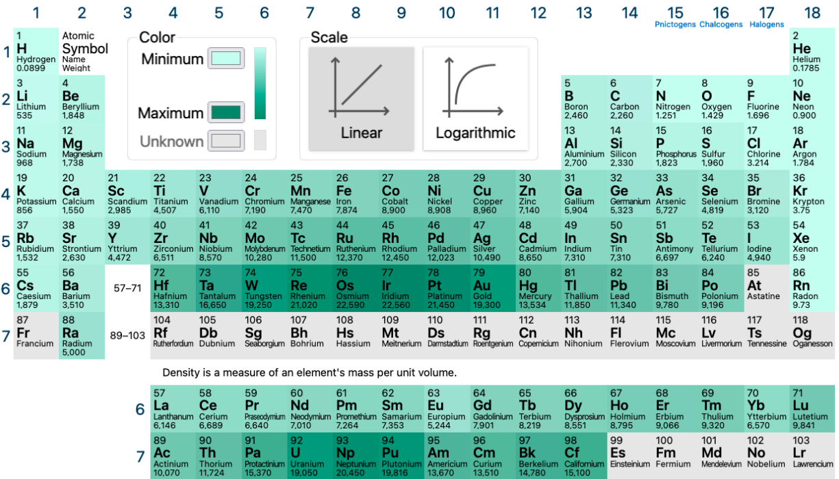
Figure 10. The densities of elements (screenshots from the ptable site ).
