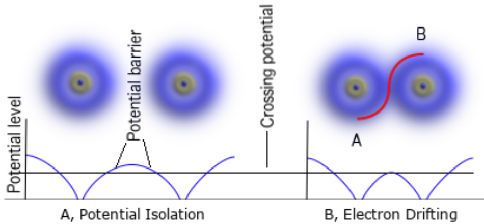
Figure 4. The difference between normal conductors and superconductors. As shown in the figure, each atomic nucleus generates an electrical field that attracts the surrounding electrons. The blue curves in the lower part of the figure represent the energy/potential level. The horizontal direction indicates the distance from the respective nucleus center, and the vertical direction is the potential scale. (A) At a considerable distance between two atoms/molecules, their electrons are separated by an energy barrier. To enable electrodrift, energy is needed to elevate electrons to the electron tunnel along the border, which is the cause of electrical resistance in conductors. (B) In superconductors, there is no such barrier as the distance between molecules is smaller, such that valence orbitals intersect electron tunnels. This distance can be reduced by increasing pressure or decreasing temperature, pushing the electron tunnel lower to overlap the valence orbitals and allowing electrons to drift from one molecule to the next without lifting energy, as illustrated by the red path A-B.
