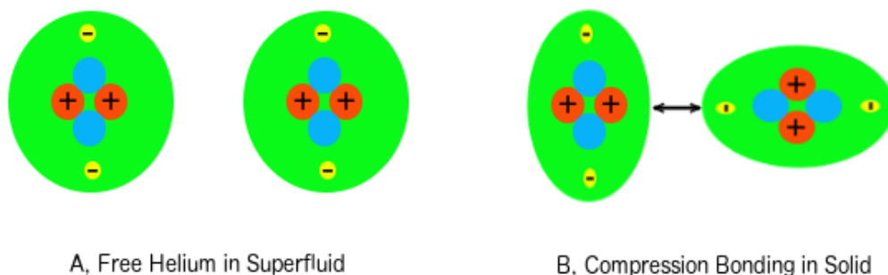
Figure 3. Compression bonds develop between helium molecules at high pressures. (A) Under normal pressures on Earth, superfluids can be obtained from liquid helium by lowering the temperature to the point where the London dispersion disappears. However, unlike most substances, solid helium cannot be produced by further reducing the temperature because there is no attraction to hold the molecules together. Pressure must be applied to obtain solid helium. (B) Under high pressures, the electron cloud of each molecule contracts along the axis through the two protons. This uneven distribution of electron density in different directions creates local electric fields, resulting in an attraction between molecules, named the compression bond. Solid helium is molecules held together by these bonds.
