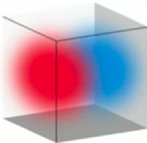
Figure 0. A quantum model of a hydrogen atom next to a proton.
