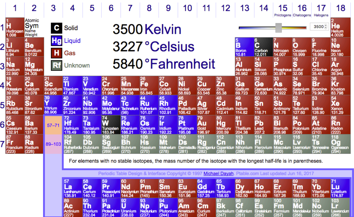
Figure 11. The states of elements at 3500 K (screenshots from the ptable site ).
