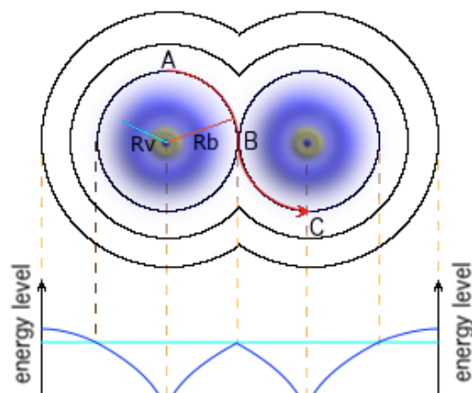
Figure 1. The concept of electron tunnel illustrated using a simple model involving a hydrogen atom adjacent to a proton. In this model, the valence electron is attracted by both its host nucleus and the neighboring proton. The electron tunnel between the hydrogen atom and the proton enables the electron to move from one to the other. In the diagram, the blue short stroke represents the radius of the valence orbital, denoted by R_v , and the red stroke indicates the radius to the border between the hydrogen atom and the proton, denoted by R_b . The contours show the orbitals at different energy levels intersecting with a plane passing through the centers of the protons. The blue curves in the lower part of the figure represent the potential level of the protons as a function of the distance from the center of each proton. An electron in the electron tunnel may drift from one proton to the other along a path at the same energy level, such as the path A-B-C.
