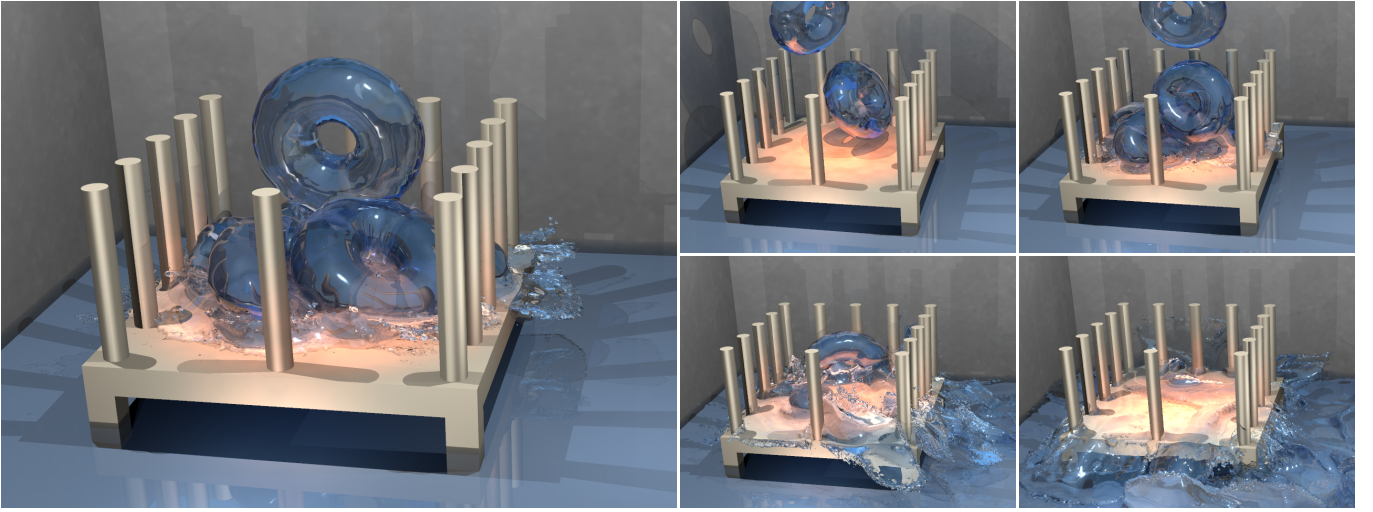
Fig. 10. Six elastic tori fall onto a hot surface causing them to quickly melt into liquid (181x61x181 grid, 160K total tetrahedra).
