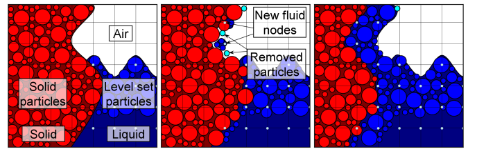
Fig. 11. A melting solid partially immersed in liquid. Particles are seeded throughout the solid with the same distribution and properties as the particle level set particles (left). As the solid melts, particles leave the solid and are converted to removed liquid particles. Some of these particles are close enough to grid nodes to convert them to liquid (middle). More liquid is generated as the solid continues melting (right).
