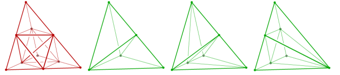
Fig. 6. Red refinement produces eight children that reside on a BCC lattice of half the size (left). Three types of green refinement are allowed in order to remove T-junctions (right).
