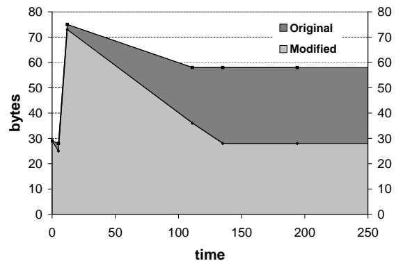
Figure 2: A comparison of the amount of tainted string data in the original Mozilla versus our modified version. Our zero-on-free string remedy reduces tainted string data by half in the steady state.
