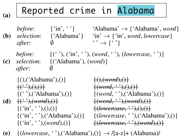
Figure 10. Regular Expression Inference. (a) The user selects text in a cell. (b) We tokenize selected and surrounding text. For clarity, the figure only includes two neighboring tokens. For each token, we generate a set of matching labels. (c) We enumerate all label sequences matching the text. (d) We then enumerate all candidate before, selection and after combinations. Patterns that do not uniquely match the selected text are filtered (indicated by strike-through). (e) Finally, we construct regular expressions for each candidate pattern.
